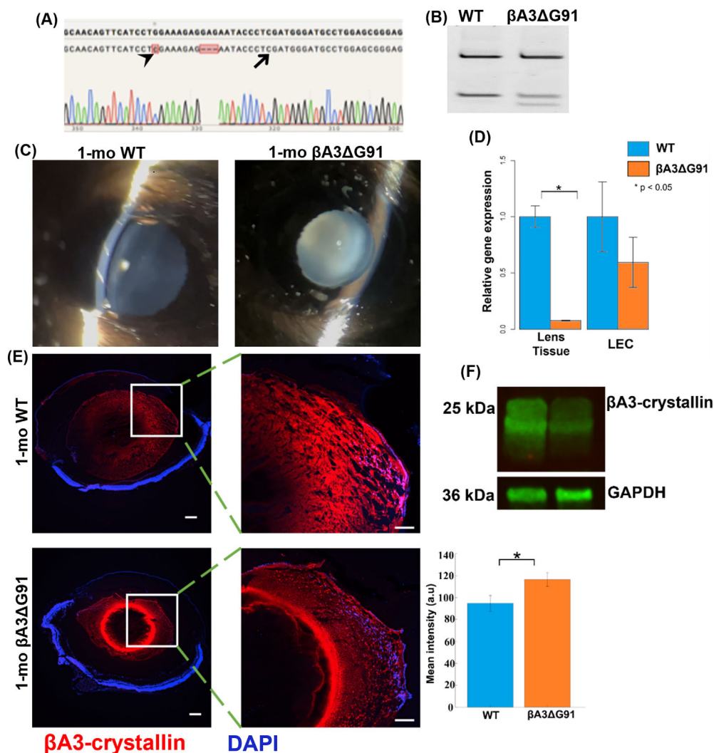
FIGURE 1. Phenotypic characterization of \beta A3\Delta G91 mice. (A) DNA from the tail was amplified with primers spanning the target region on exon 4 of the CRY\beta A1/A3 gene. Sequence analysis verifies the GAG deletion that leads to the glycine-91 deletion and the additional silent mutation, creating a second TaqI restriction site for genotyping (black arrowhead). (B) Genotyping results show two and three bands for WT and \beta A3\Delta G91 mice, respectively. (C) Slit-lamp photographs of 1-month-old mice revealed that the mutant mice had a dense nuclear cataract (right) whereas the WT mice had a clear lens. (D) Significantly lower levels of CRY\beta A1 mRNA seen in the whole lens tissue is demonstrated by RT-qPCR analysis (left graph). (E) IHC revealed a relatively smaller lens with puncta in the outer cortex, and a bright ring-like pattern formed in the inner cortex of \beta A3\Delta G91 lenses (shown in 4 \times and 20 \times , respectively). Scale bar: 200 \mu m. * P < 0.05 versus age-matched WT. (F) Western blots of RIPA-soluble lens homogenates probed with the anti- \beta A3 -crystallin antibody show a decreased expression of the protein in \beta A3\Delta G91 lenses relative to WT lenses. GAPDH was used as a loading control.
