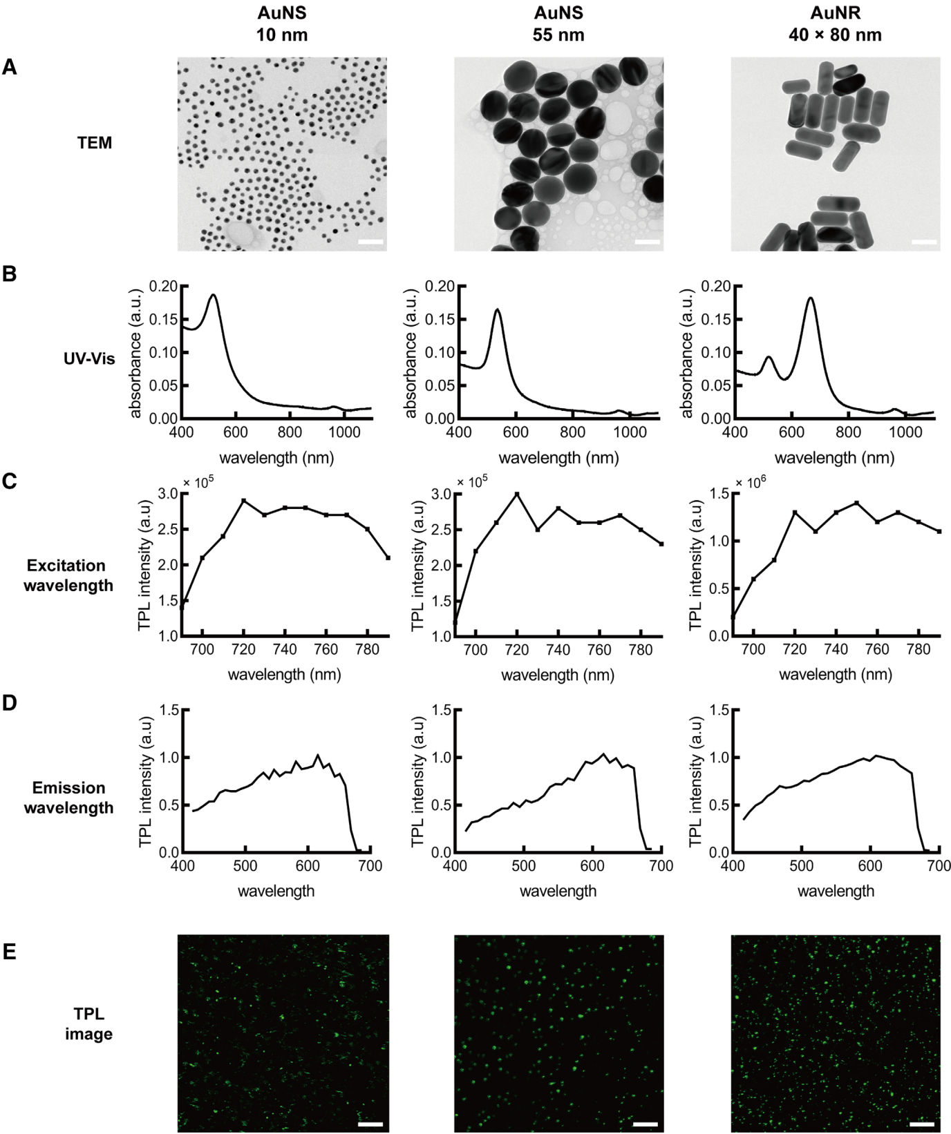
Figure 3. Characterization of AuNPs. (A) Representative TEM images of 10-nm AuNSs ( left ), 55-nm AuNSs ( middle ), and 40 × 80-nm AuNRs ( right ). Scale bar: 50 \mu m. (B) UV-Vis graph of 10-nm AuNSs ( left ), 55-nm AuNSs ( middle ), and 40 × 80-nm AuNRs ( right ). (C) Excitation wavelength graph of 10-nm AuNSs ( left ), 55-nm AuNSs ( middle ), and 40 × 80-nm AuNRs ( right ). (D) Emission wavelength graph of 10-nm AuNSs ( left ), 55-nm AuNSs ( middle ), and 40 × 80-nm AuNRs ( right ). (E) Representative TPL image of 10-nm AuNSs ( left ), 55-nm AuNSs ( middle ), and 40 × 80-nm AuNRs ( right ). Scale bar: 10 \mu m.
